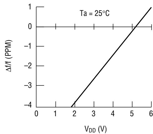
Figure 3 Frequency Deviation (PPM) vs Voltage
