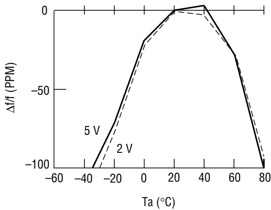
Figure 2 Frequency Deviation (PPM) vs Temperature
